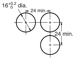
Square A165□-A Round A165□-T (Top View)
