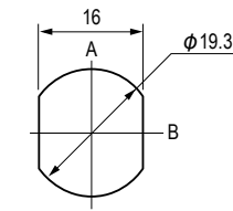
取付穴図 Holes for Installation
