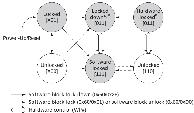
Figure 6: Block Locking State Diagram
