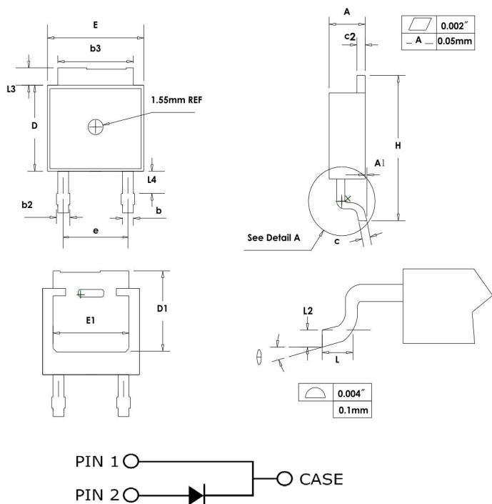
Package TO-252-2
