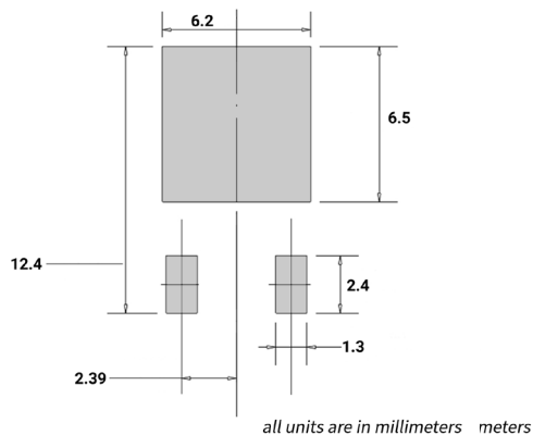
TO-252-2
