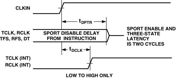
Figure 21. Serial Ports
