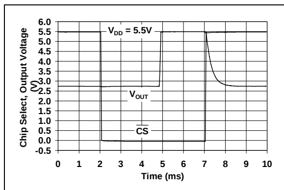
FIGURE 2-39: Chip Select (CS) Step Response (MCP6548 only).
