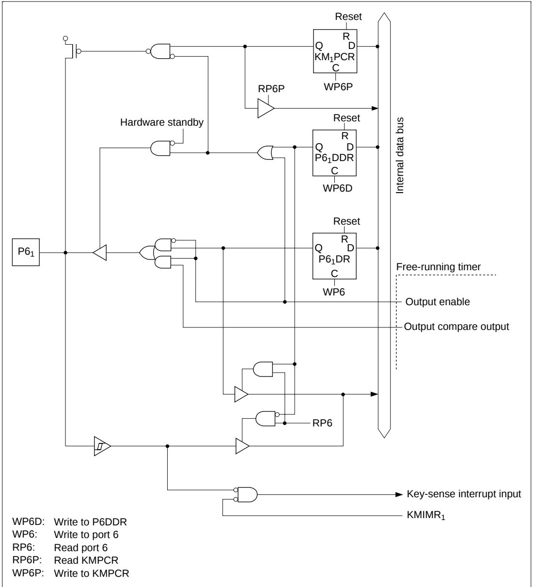
Figure C.6 (b) Port 6 Block Diagram (Pin P6 I )
