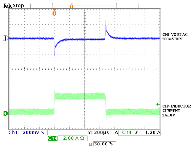
Figure 6. Transient Response
