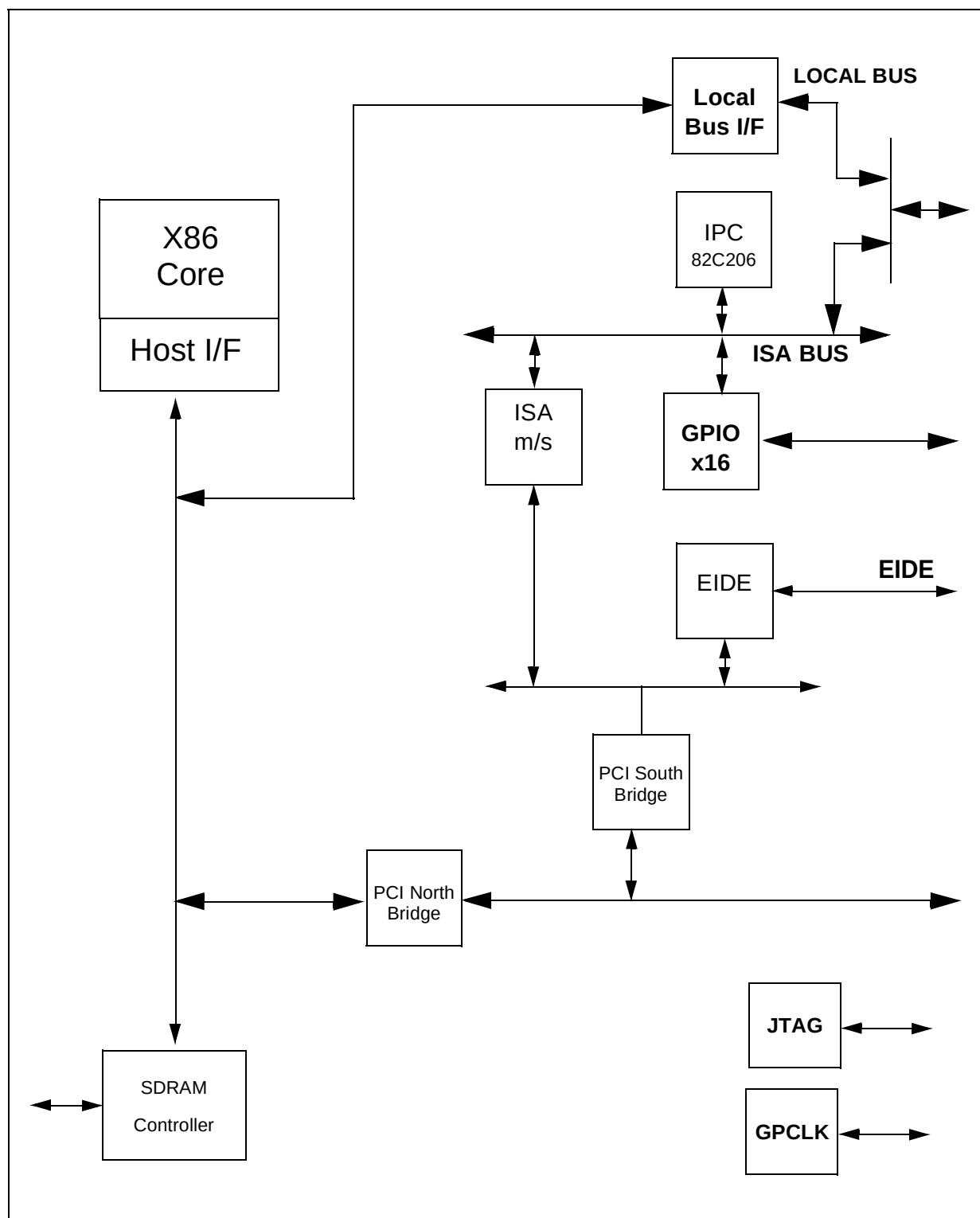
Figure 1-1. Functional description.
