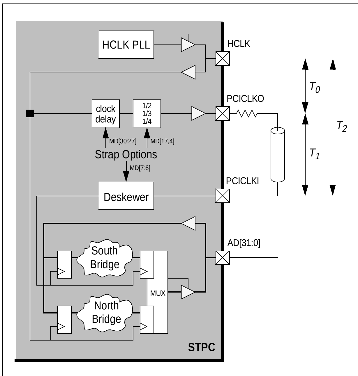
Figure 6-21. Clock Scheme
