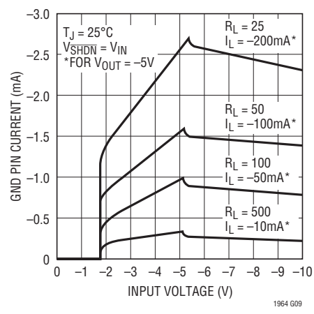
LT1964-5 GND Pin Current
