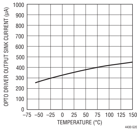
Opto Driver Output Sink Current vs Temperature
