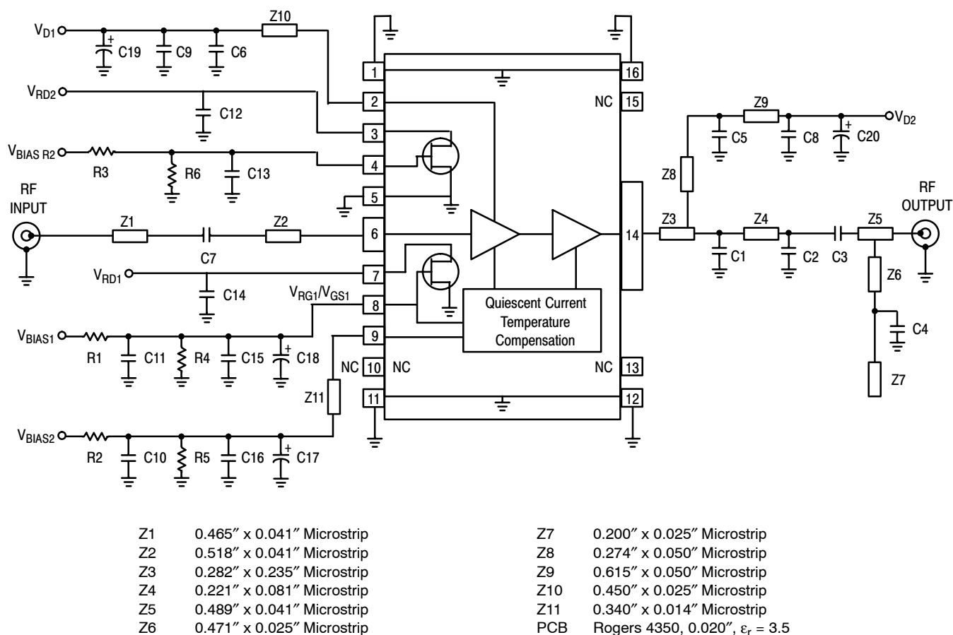
Figure 3. MW5IC2030MBR1(GMBR1) Test Circuit Schematic
