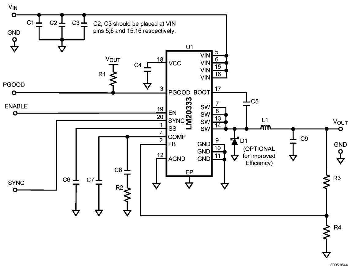
FIGURE 14. Typical Application Schematic
