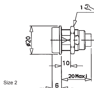
SE : Sealed Sealed Panel Mount Cable Receptacle
