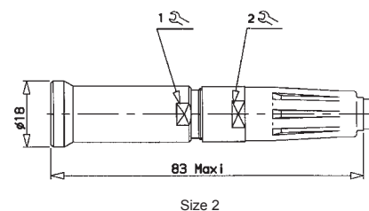
HH : Sealed Front Mount Receptacle
