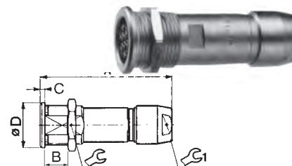
SR : Front Mount Cable Receptacle
