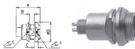
EP: Rear Mount
