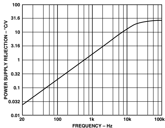
TPC 4. Power Supply Rejection vs. Frequency
