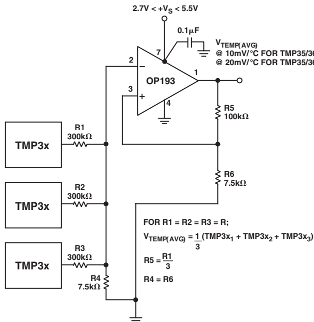
Figure 6a. Configuring Multiple Sensors for Average Temperature Measurements
