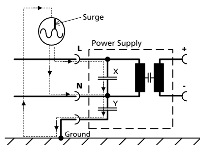
Fig. 23-5 Earthed input
