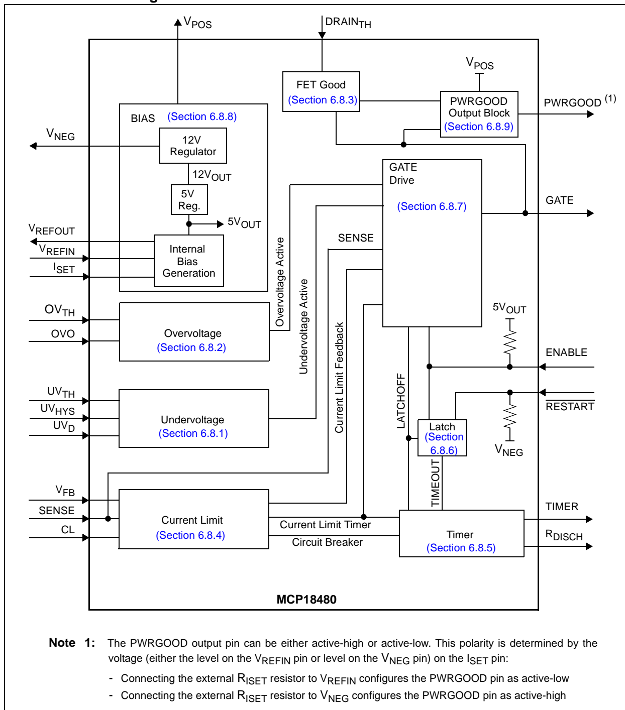
MCP18480 Block Diagram
