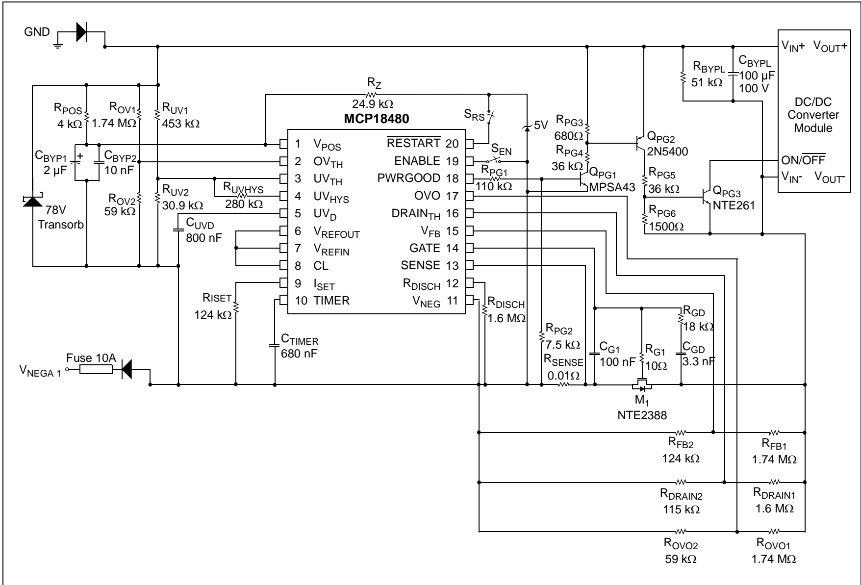
FIGURE B-2: Typical Operating Circuit for Telecom Applications with Active-Low Power Module - Foldback Current Limit Enabled.
