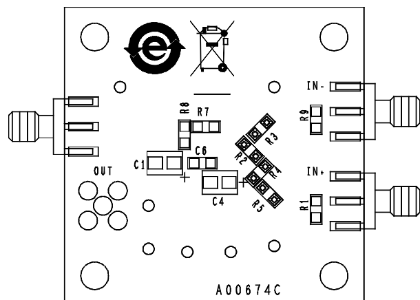
Figure 6. Board Assembly Drawing, Circuit Side
