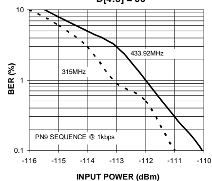
BER vs. Input Power D[4:3] = 00
