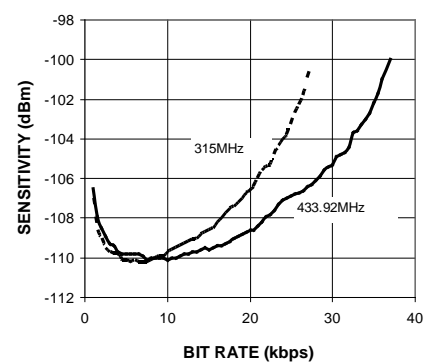
Sensitivity at 1% BER D[4:3] = 10
