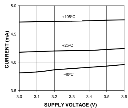
Current vs. Supply Voltage f_{RF} = 315MHz
