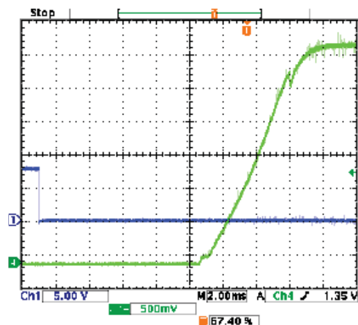
On/Off ENABLE DELAY ( V_{in}=48V , V_{out}=nom , I_{out}=7.5A , C_{load}=0\mu F , T_a=+25^\circ C , ScopeBW=20Mhz) Trace 1= Enable. Trace 4=Vout
