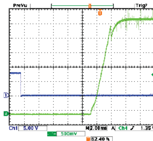
On/Off ENABLE DELAY ( V_{in}=48V , V_{out}=nom , I_{out}=7.575mA , C_{load}=0\mu F , T_a=+25^\circ C , ScopeBW=20Mhz) Trace 1= Enable. Trace 4=Vout
