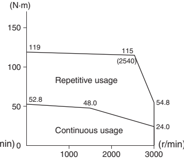
R88M-W7K515T (7.5 kW)
