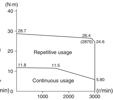
R88M-W7K515T (7.5 kW)
