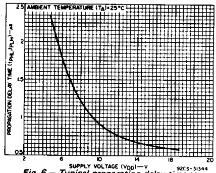
Fig. 6 - Typical propagation delay time as a function of supply voltage ( \phi_I to y or y + d out vs. V_{DD} ).
