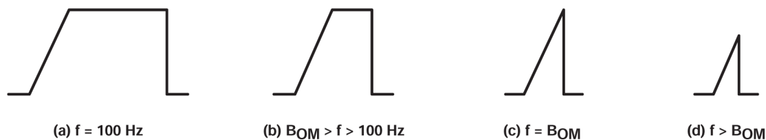
Figure 6-5. Full-Power-Response Output Signal
