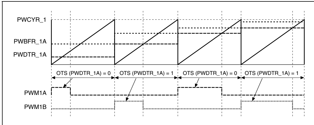
Figure 13.10 PWM Channel 1 Operation
