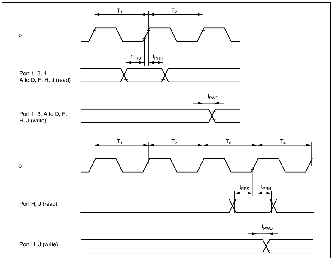
Figure 21.6 I/O Port Input/Output Timing
