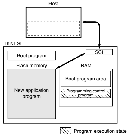
Figure 16.3 Boot Mode
