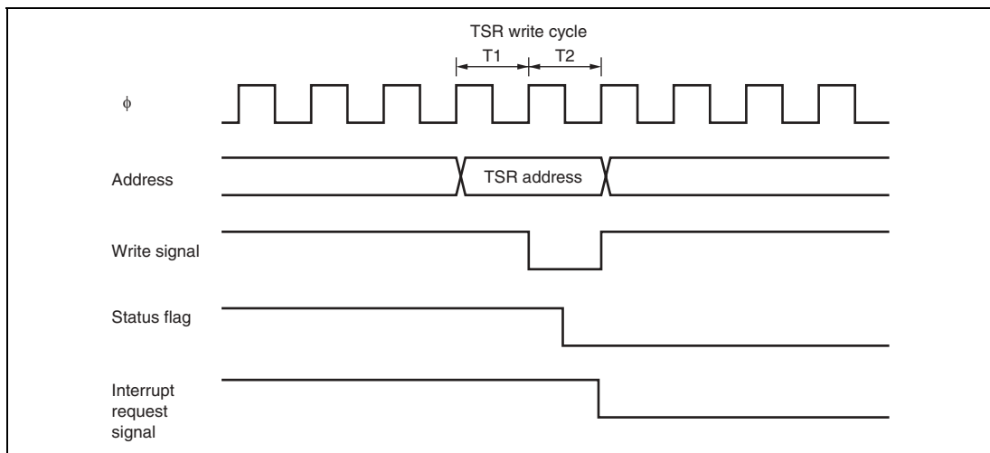
Figure 8.39 Timing for Status Flag Clearing by CPU
