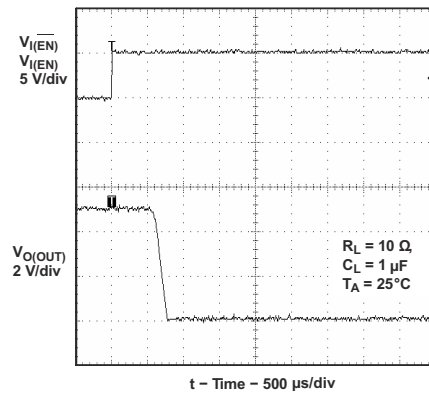
Figure 9-19. Turnoff Delay and Fall Time with 1-µF Load
