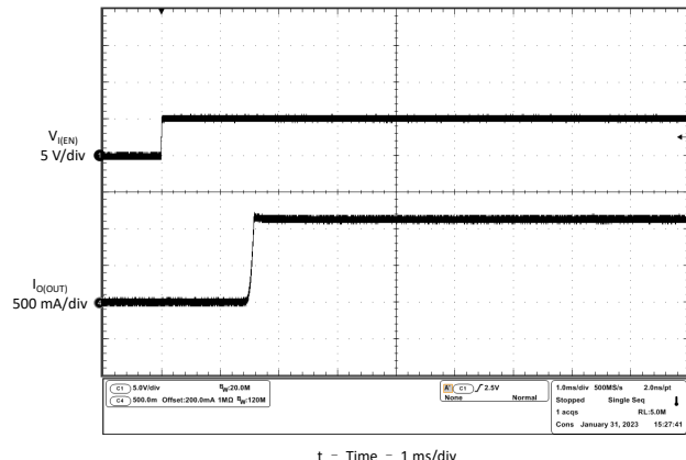
Figure 6-42. Short-Circuit Current, Device Enabled Into Short
