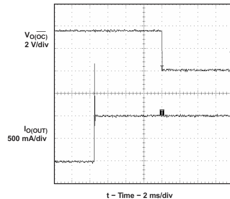
Figure 9-10. 2- \Omega Load Connected to Enabled Device
