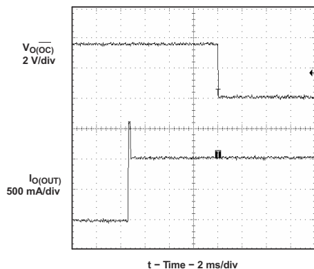
Figure 9-33. 3- \Omega Load Connected to Enabled Device
