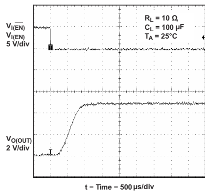
Figure 9-20. Turnon Delay and Rise Time With 100-µF Load
