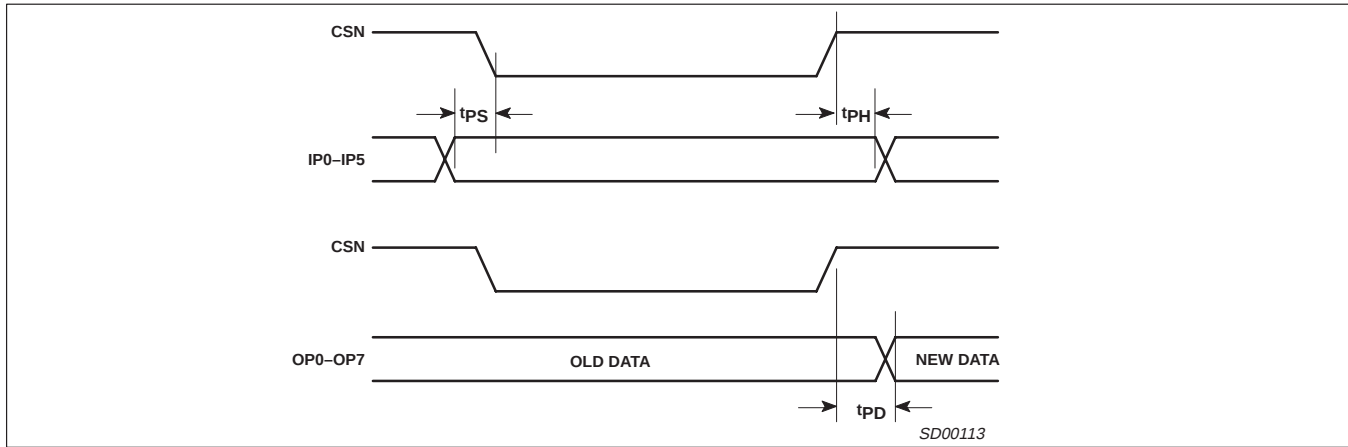
Figure 7. Port Timing
