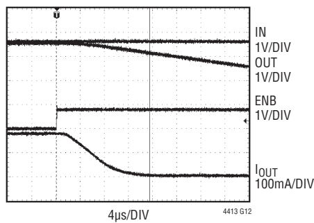
ENB Turn-Off, 16 \mu s to Disconnect IN from 180mA Load
