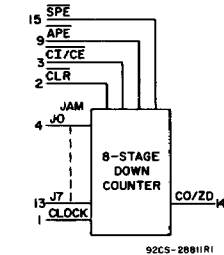
8-Stage Presettable Synchronous Down Counter CD40102B (File No. 984) 2-Decade BCD CD40103B (File No. 984) 8-Bit Binary
