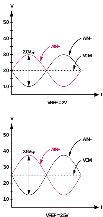
FIGURE 27. RELATIONSHIP BETWEEN VREF AND FULL-SCALE RANGE
