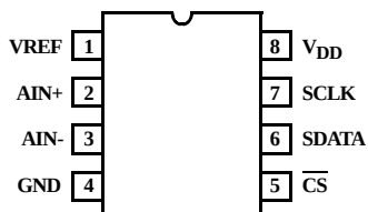
ISL26712/10/08 (8 LD TDFN) TOP VIEW
