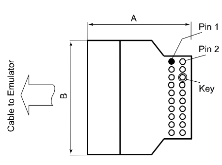
FIGURE 31 Dimensions of the 20-pin CTI20 probe. Top view. A = 27.0 mm (1.06 in.) B = 17.8 mm (0.70 in.).
