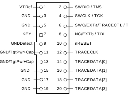
FIGURE 41 The Cortex20 pinout of the Cortex side of the ADA-ETM-SWD20 probe. Top view.
