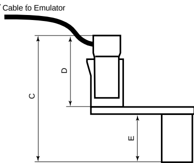
FIGURE 20 The dimensions of the 14-pin JTAGjet probe for OMAP and TMS320 DSP. Side view. C = 24 mm (.95 in.), D = 14.7 mm (0.58 in.), E = 8.5 mm (0.34 in.).
