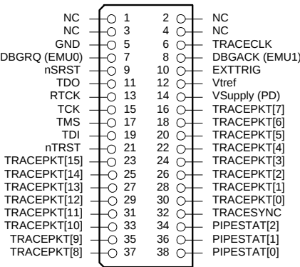
FIGURE 42 The ETM32 pinout of the ETM side of the ADA-ETM-SWD20 probe. Top view.
