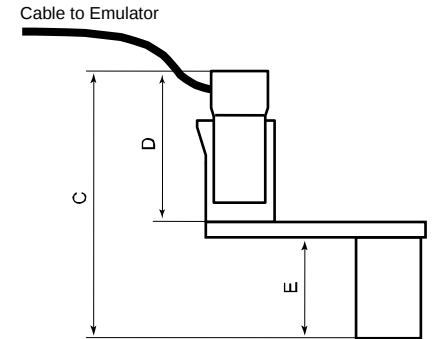
FIGURE 32 Dimensions of the 20-pin CTI20 probe. Side view. C = 23.0 mm (.91 in.), D = 12.5 mm (0.49 in.), E = 6.4 mm (0.25 in.).
