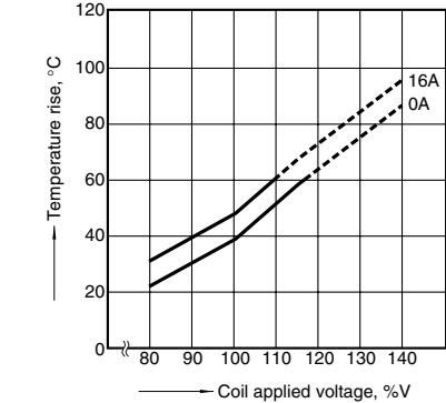
2-(1). Coil temperature rise (1 Form C/AC and 1 Form A/AC types) Measured portion: Inside the coil Ambient temperature: 70°C 158°F
