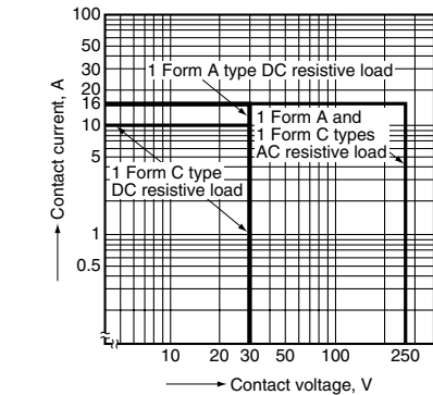
1-(1). Max. switching capacity (1 Form C and 1 Form A)
