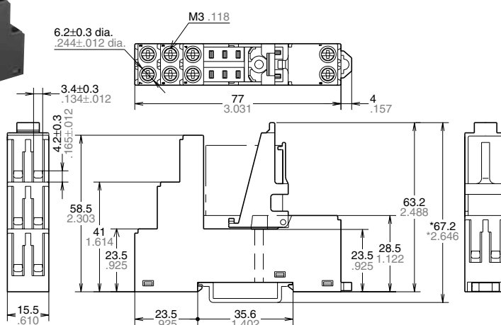
External dimensions
