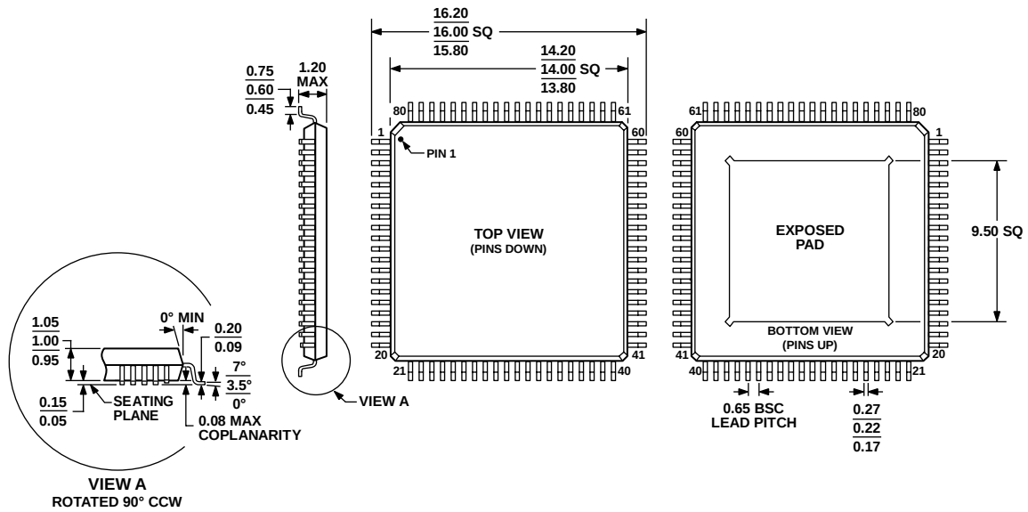
Figure 68. 80-Lead Thin Quad Flat Package, Exposed Pad [TQFP_EP] (SV-80-4)
