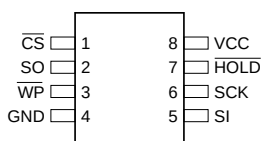
8-lead SOIC
