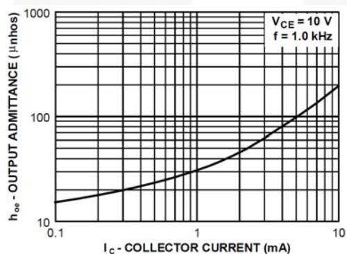
Figure 14. Output Admittance
