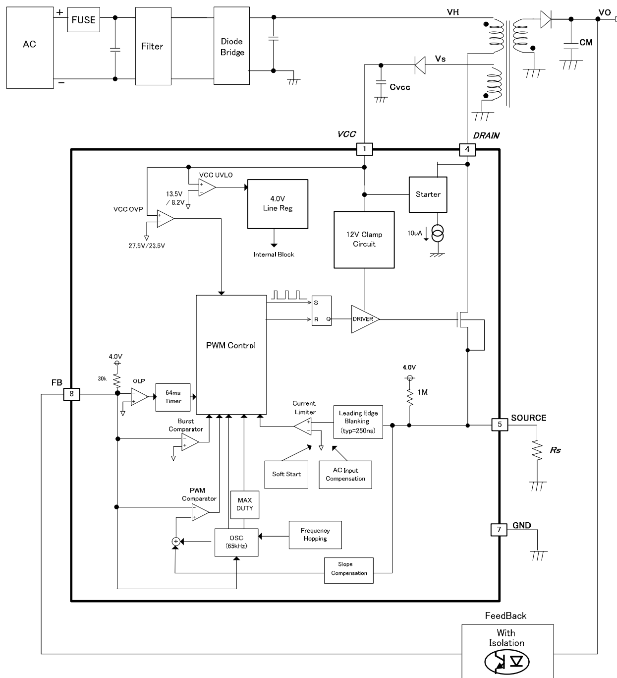
Figure 3. Block Diagram
