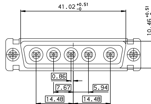
DETAIL OF PRESS FIT Scale: 3
