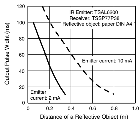
Fig. 14 - Distance Characteristic of a Typical Reflective Sensor Using the TSSP77P38
