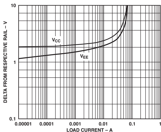
Figure 25. OPA627 Dropout from \pm 15\text{ V} vs. Load Current
