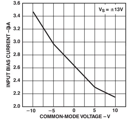
TPC 6. Input Bias Current vs. Common-Mode Voltage
