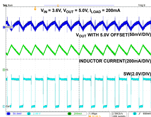
FIGURE 18. PWM WAVEFORM
