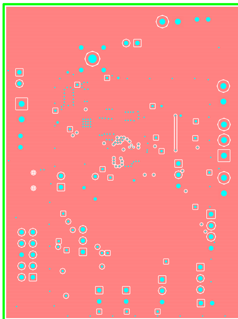
Figure 6. Layer 4
