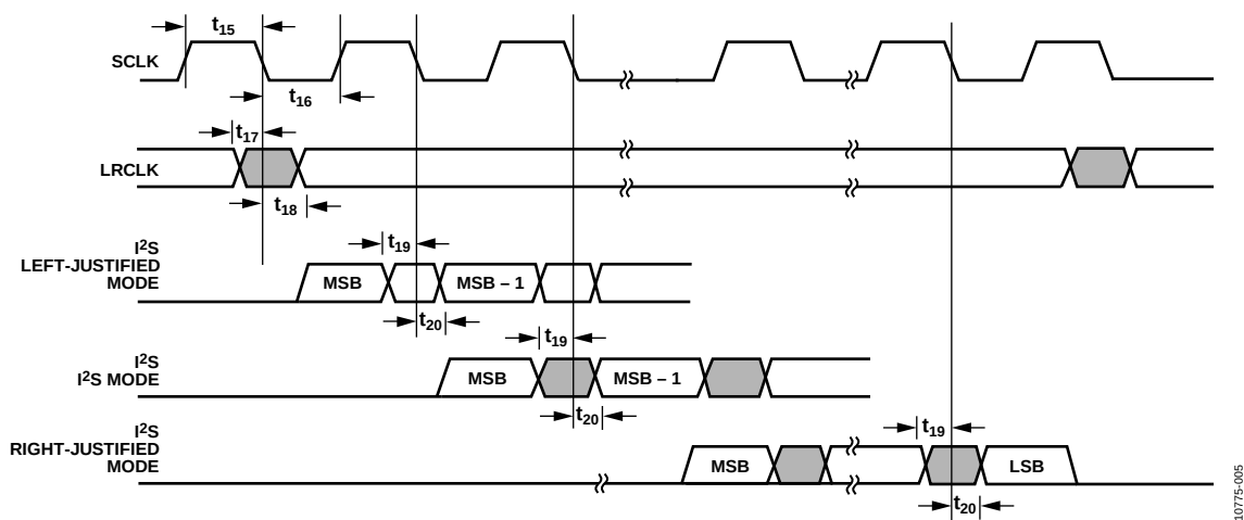
Figure 5. I²S Timing
