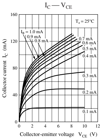
Characteristics charts of UNR1212
