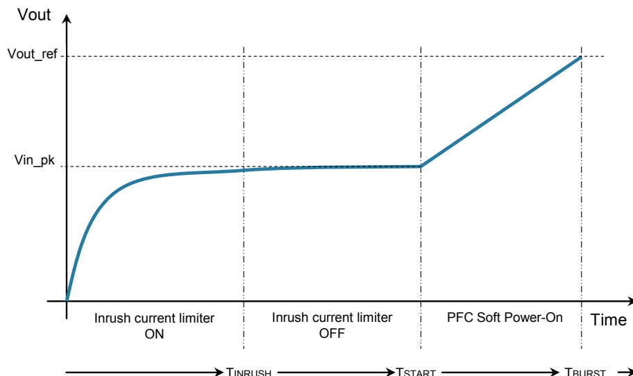
Figure 14. Start-Up sequence
