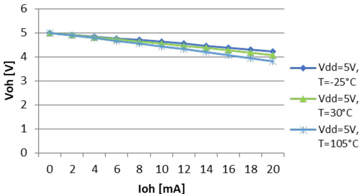
Figure 28. V_{OH} fast I/Os pins
