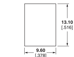
Recommended Panel Cutout Max. Panel Thk. 1.7 [0.067]
