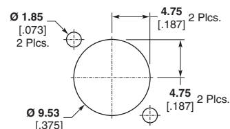
Recommended Panel Cutout Max. Panel Thk. 1.70 [0.067]
