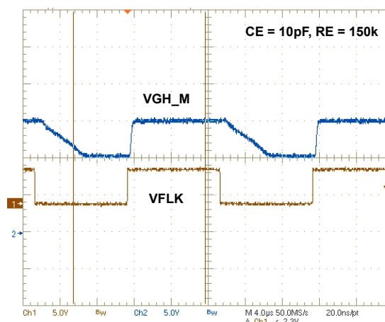
FIGURE 10. GPM CIRCUIT WAVEFORM
