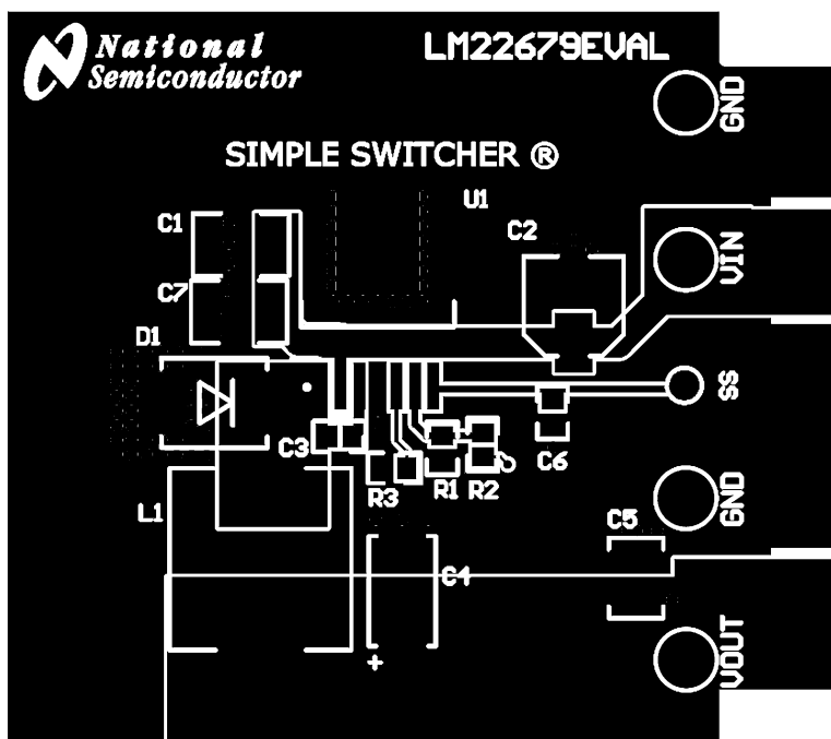
Figure 6. Top Layer
