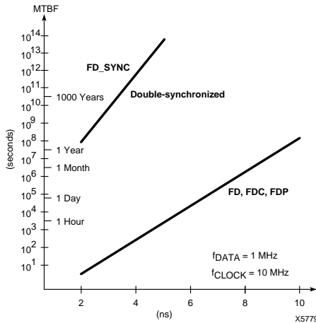
Figure 19: Metastable MTBF
