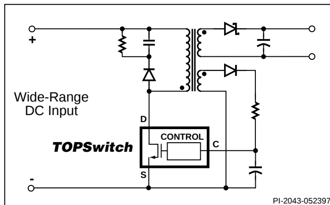
Figure 1. Typical Application.
