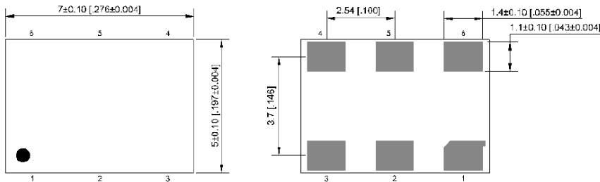
External Dimensions
