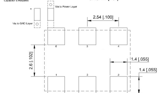
Recommended Solder Pad Layout units: mm[inch]
