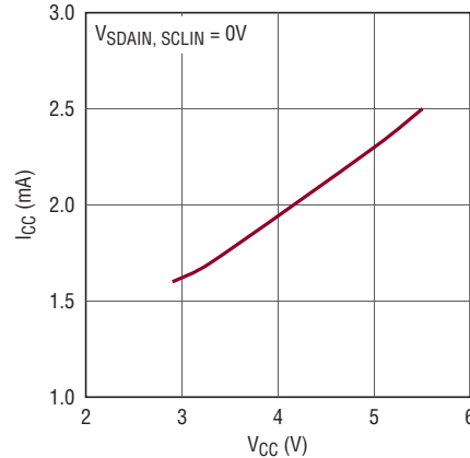
I_{CC} Disabled (ENABLE1-4 Low) Current vs Supply Voltage
